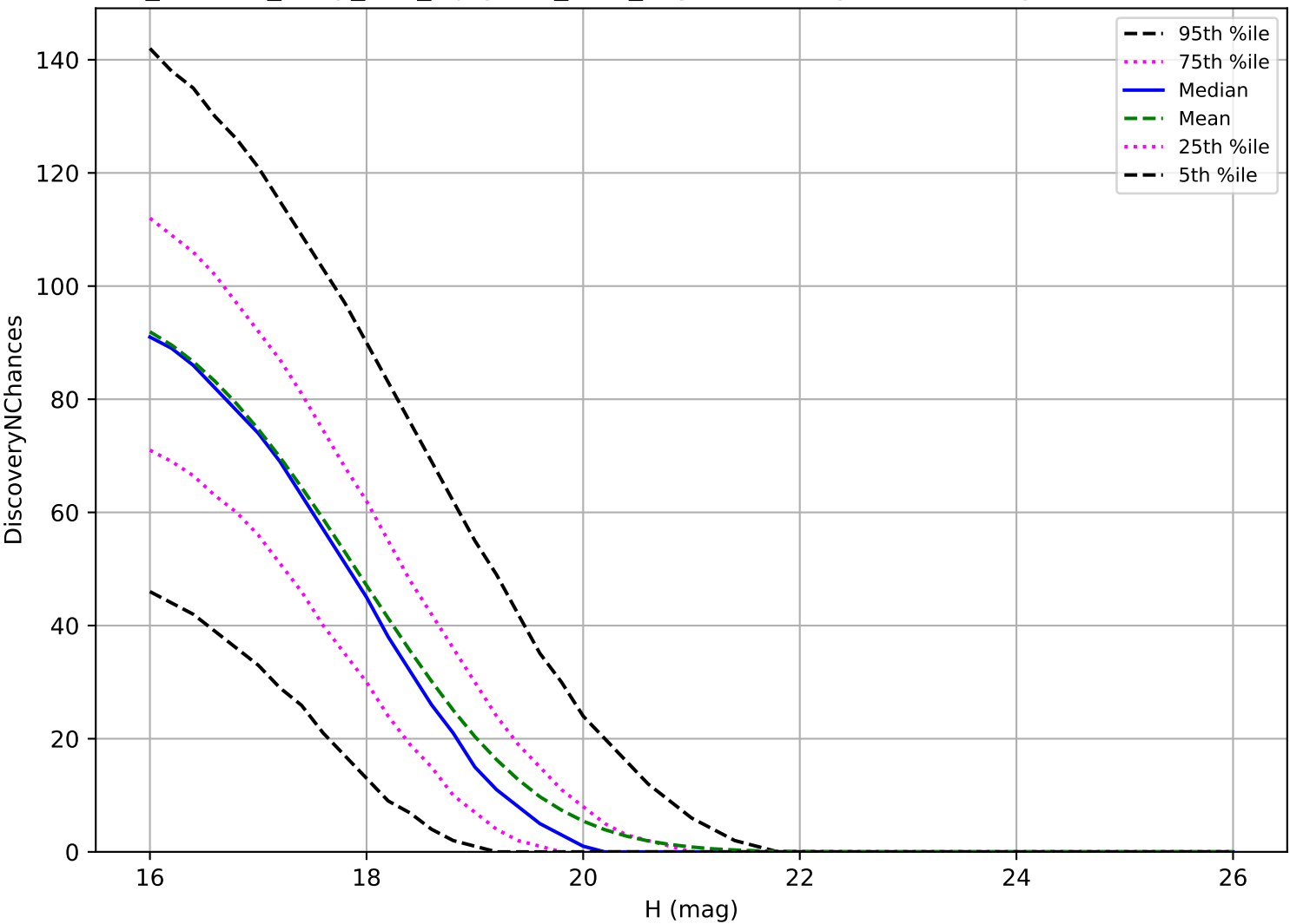
roll_uniform_early_half_mjdp180_v3.4_10yrs: MBA 3 pairs in 15 nights detection loss
