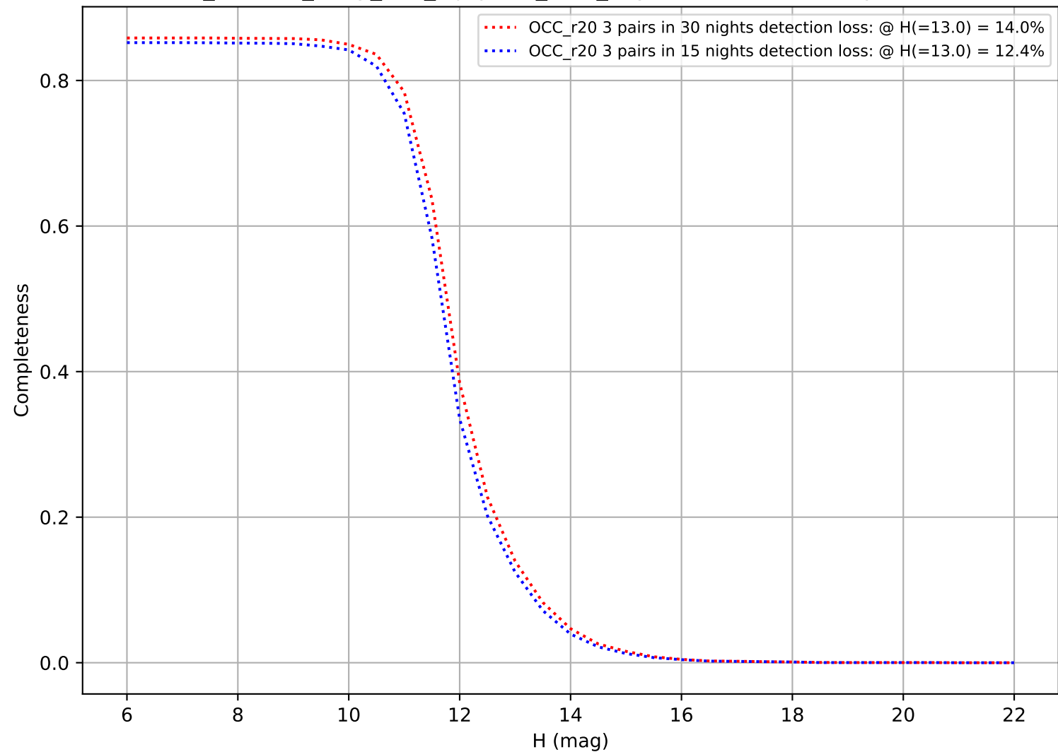
roll_uniform_early_half_mjdp180_v3.4_10yrs: DifferentialCompleteness
