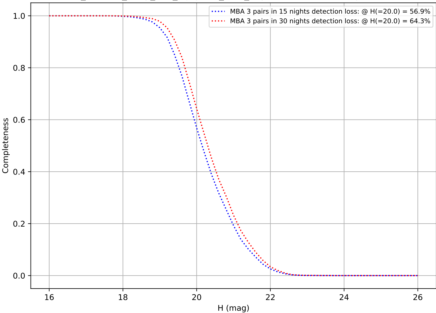
roll_uniform_early_half_mjdp180_v3.4_10yrs: DifferentialCompleteness
