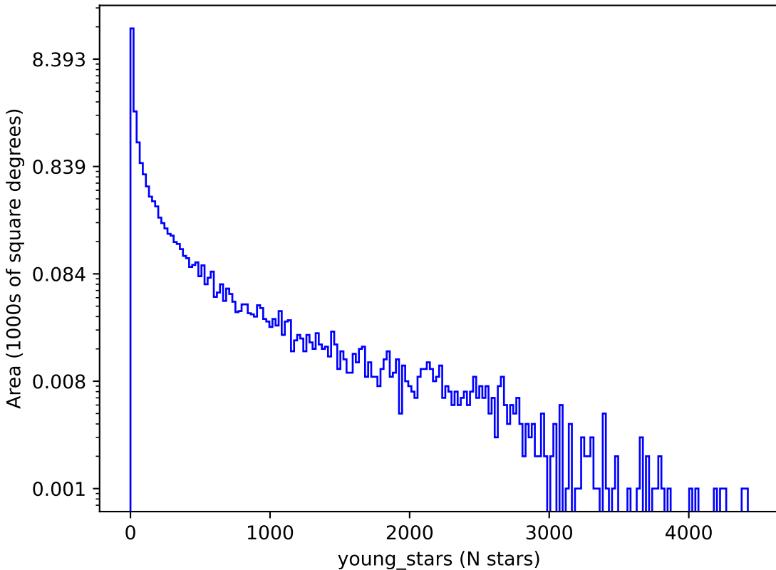
roll_uniform_early_half_mjdp180_v3.4_10yrs : young_stars
