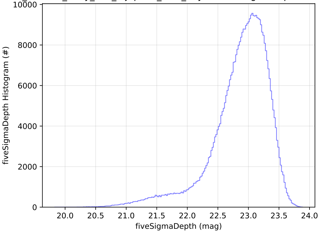
roll_uniform_early_half_mjdp180_v3.4_10yrs z: fiveSigmaDepth Histogram
