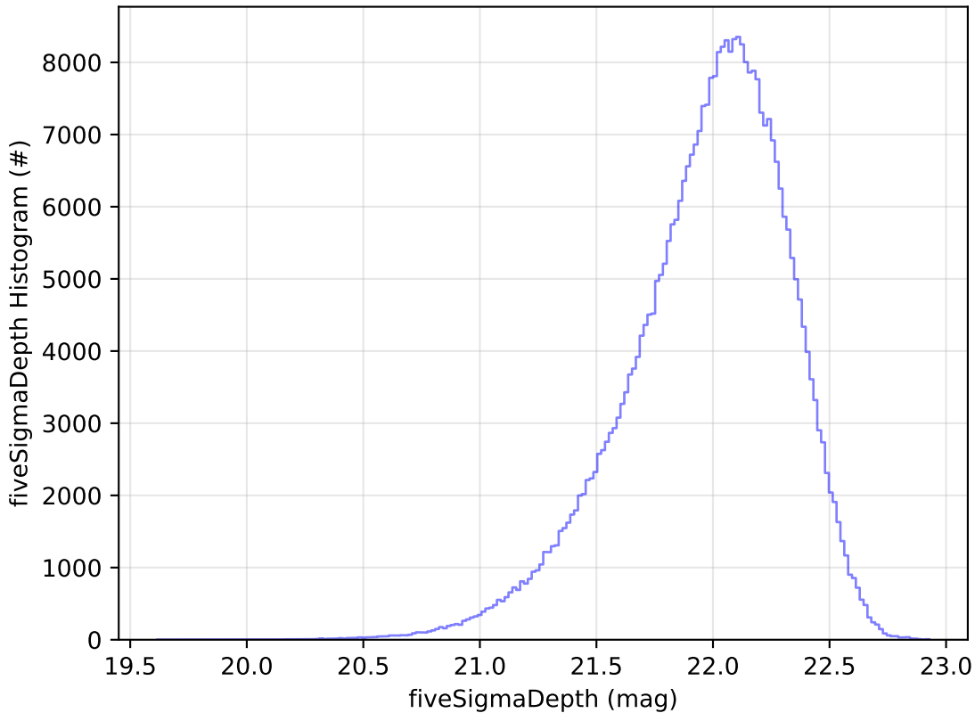
roll_uniform_early_half_mjdp180_v3.4_10yrs y: fiveSigmaDepth Histogram
