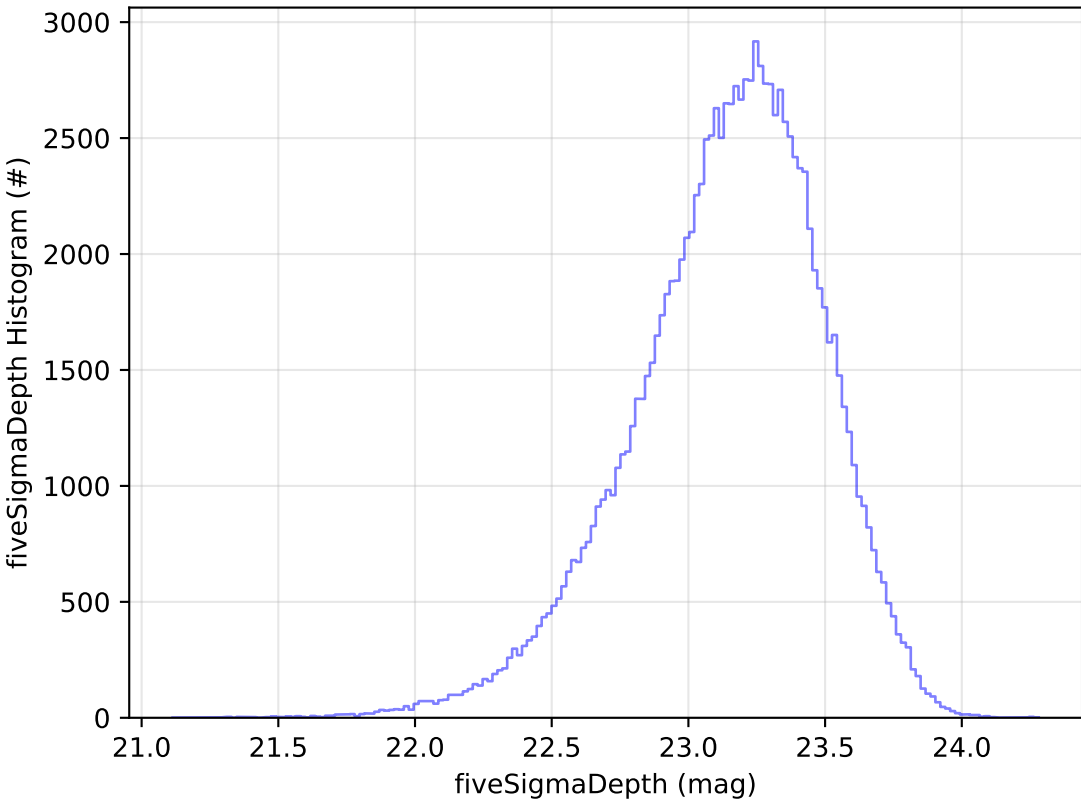
roll_uniform_early_half_mjdp180_v3.4_10yrs u: fiveSigmaDepth Histogram
