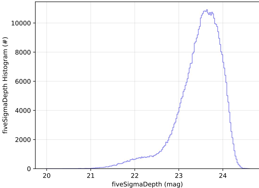
roll_uniform_early_half_mjdp180_v3.4_10yrs i: fiveSigmaDepth Histogram
