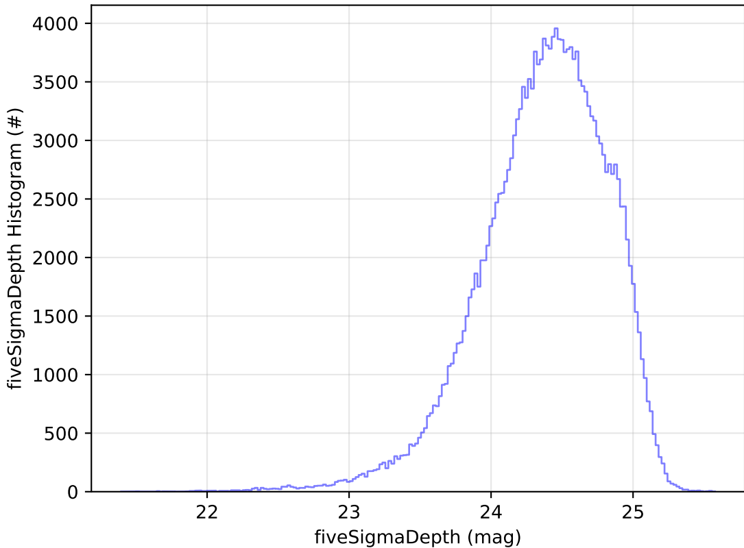
roll_uniform_early_half_mjdp180_v3.4_10yrs g: fiveSigmaDepth Histogram
