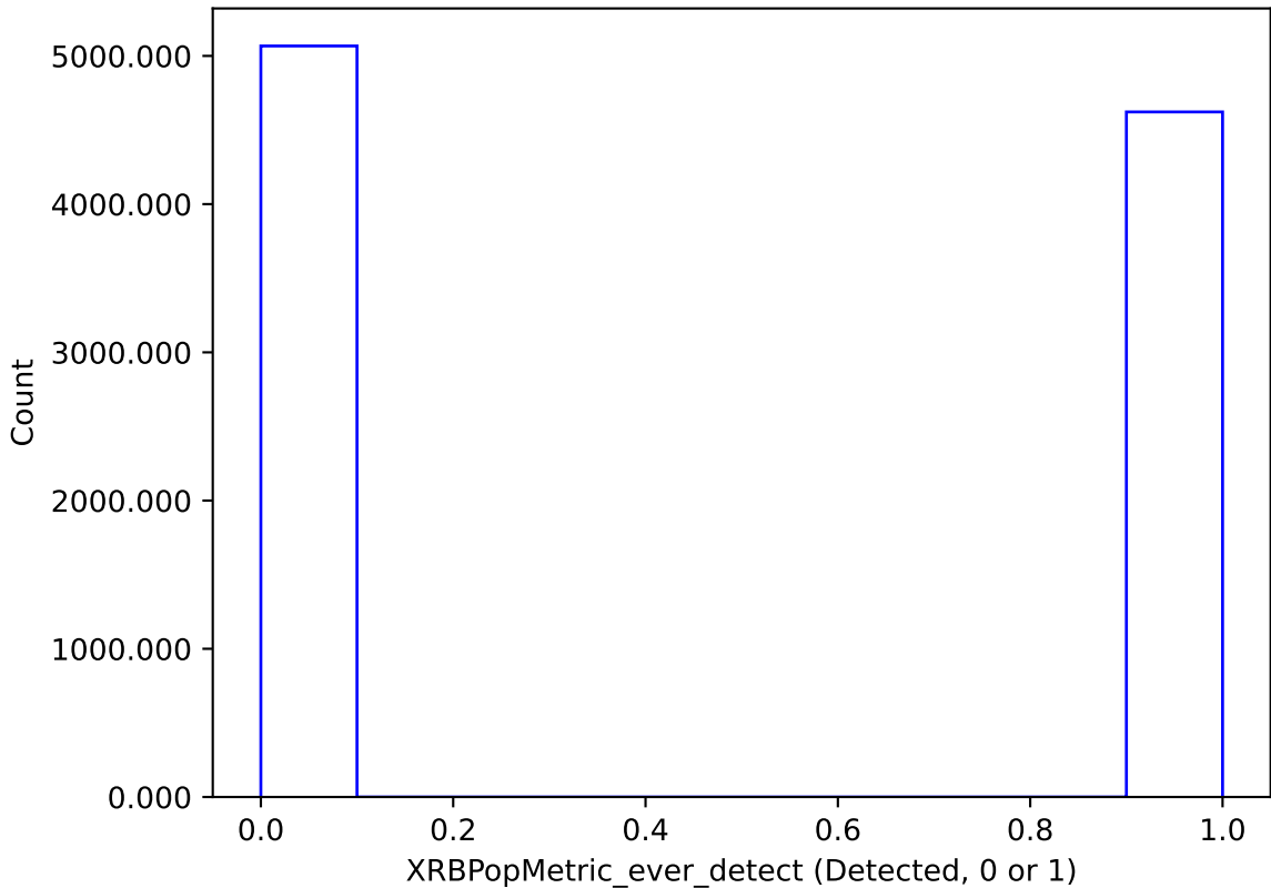
roll_uniform_early_half_mjdp180_v3.4_10yrs : XRBPopMetric_ever_detect
