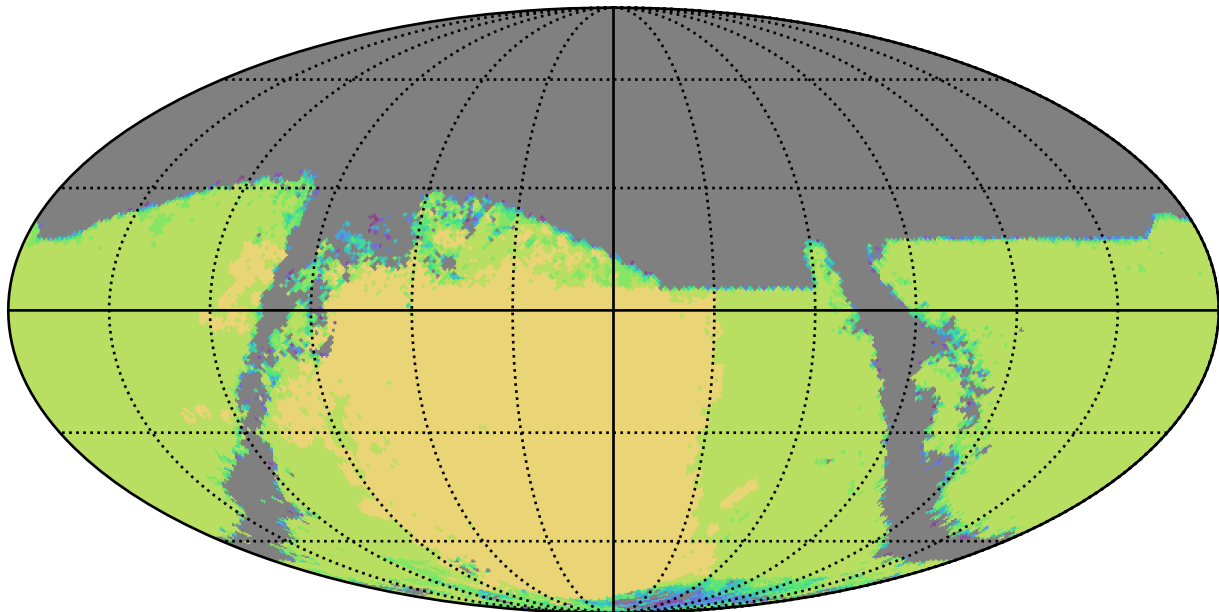
roll_uniform_early_half_mjdp180_v3.4_10yrs : TDC_campaign
