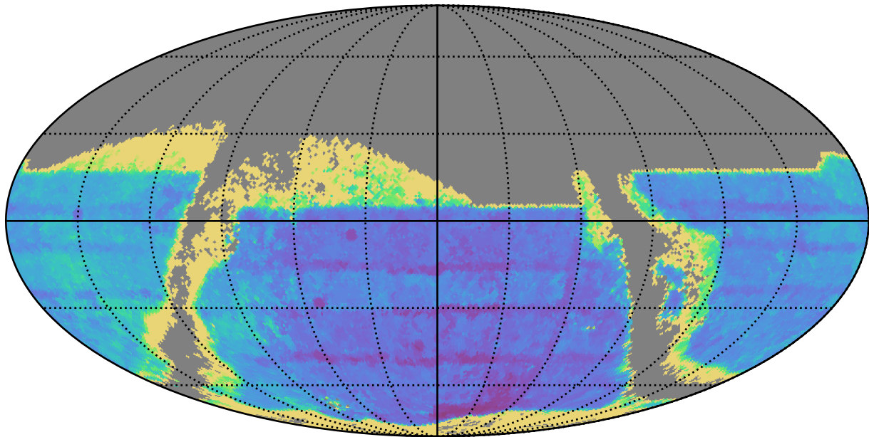
roll_uniform_early_half_mjdp180_v3.4_10yrs : TDC_accuracy
