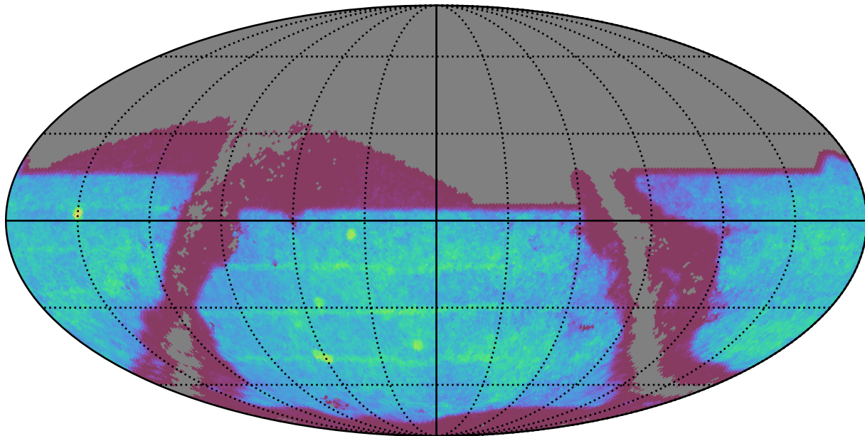
roll_uniform_early_half_mjdp180_v3.4_10yrs : SNSLMetric
