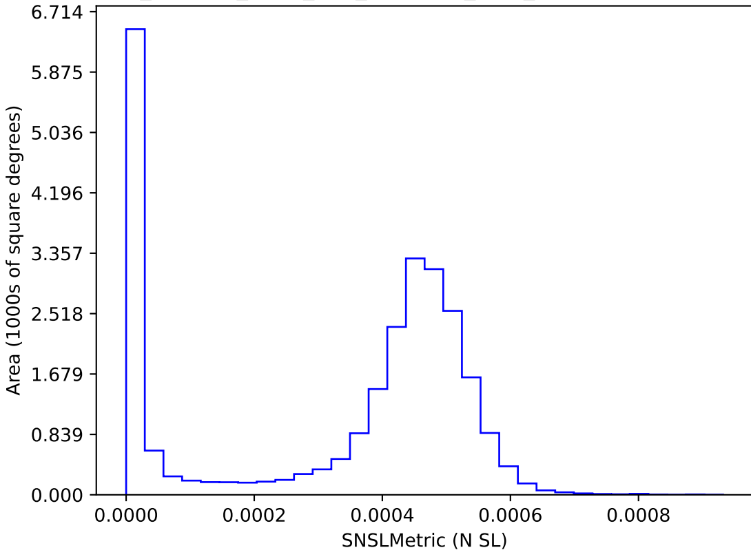
roll_uniform_early_half_mjdp180_v3.4_10yrs : SNSLMetric
