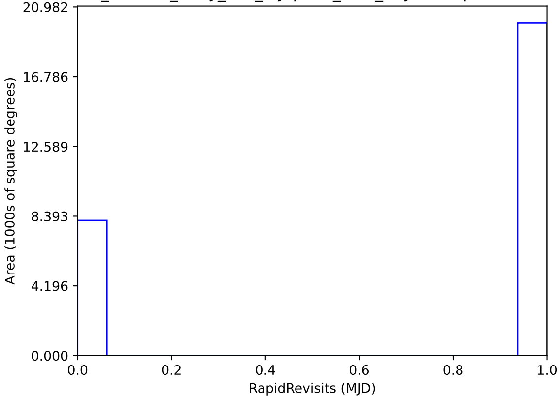
roll_uniform_early_half_mjdp180_v3.4_10yrs : RapidRevisits
