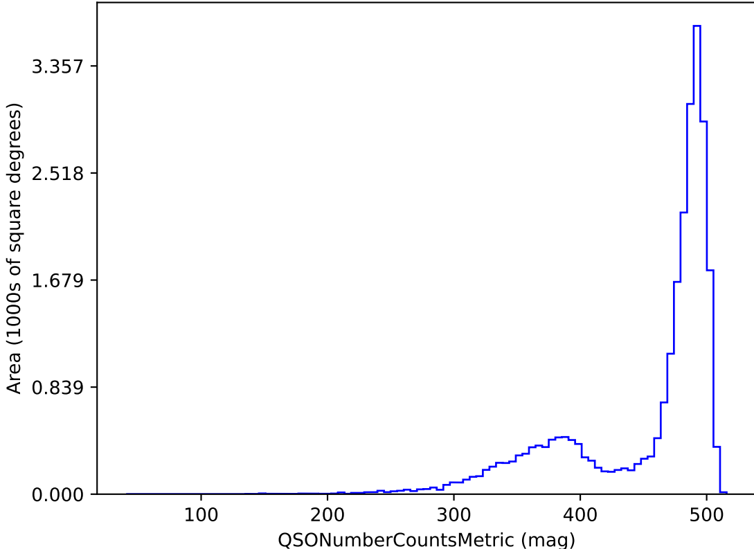
roll_uniform_early_half_mjdp180_v3.4_10yrs z band and non-DD: QSONumberCountsMetric
