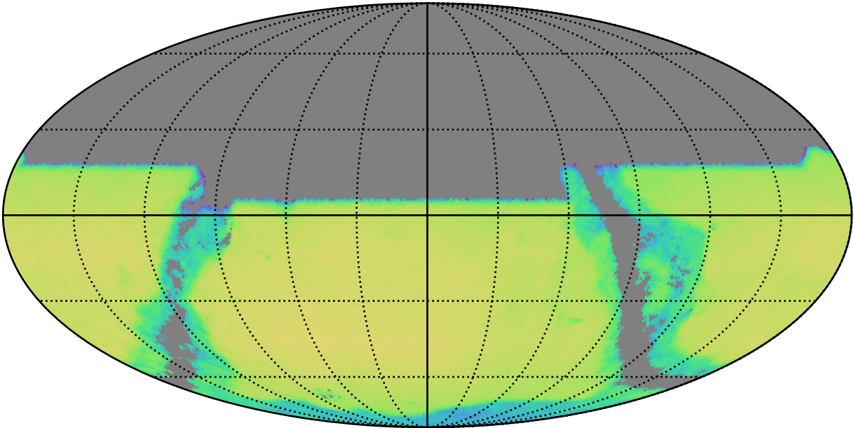
roll_uniform_early_half_mjdp180_v3.4_10yrs y band and non-DD: QSONumberCountsMetric
