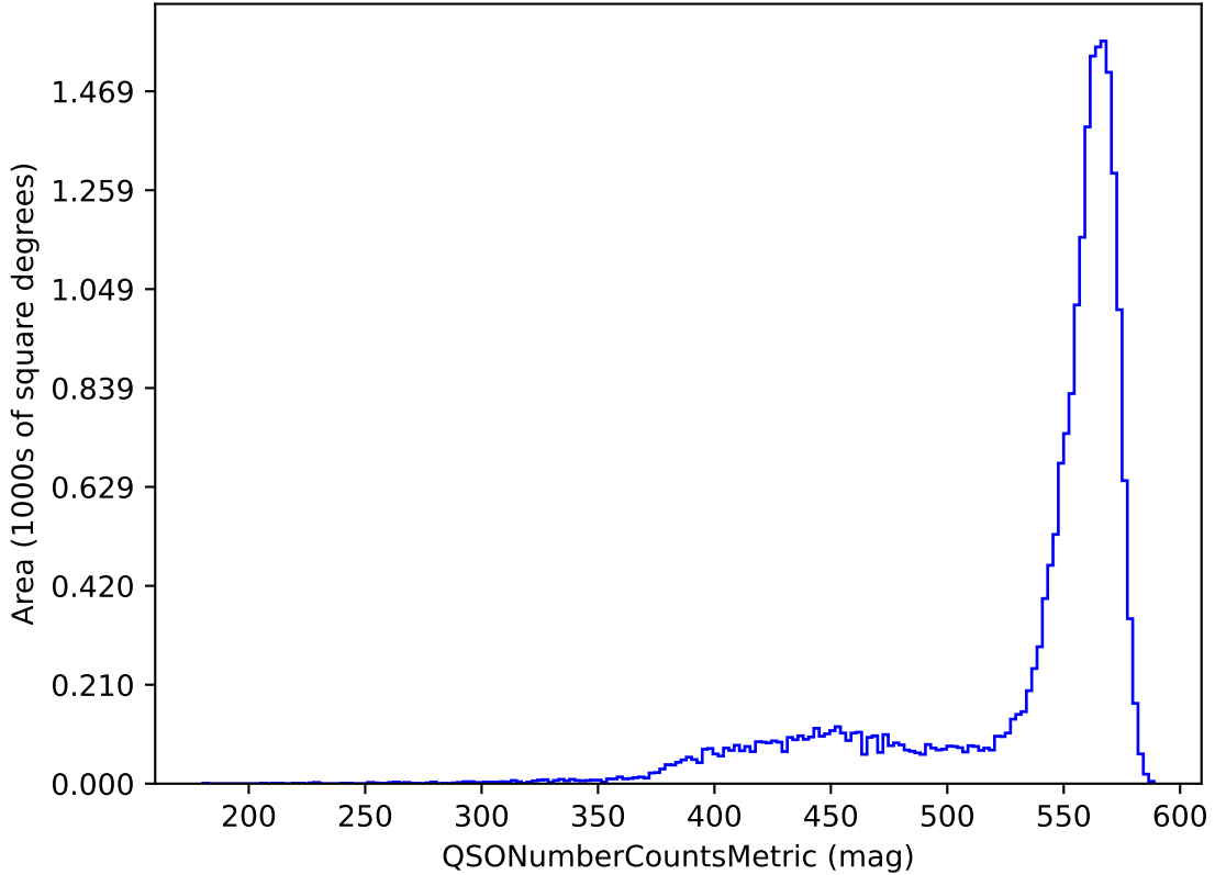
roll_uniform_early_half_mjdp180_v3.4_10yrs y band and non-DD: QSONumberCountsMetric
