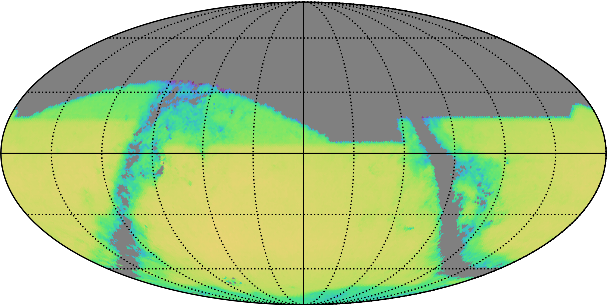
roll_uniform_early_half_mjdp180_v3.4_10yrs r band and non-DD: QSONumberCountsMetric
