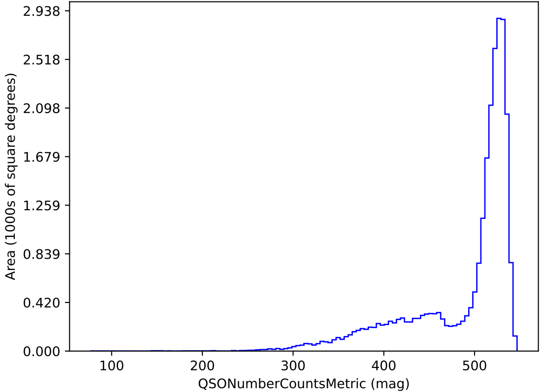
roll_uniform_early_half_mjdp180_v3.4_10yrs r band and non-DD: QSONumberCountsMetric
