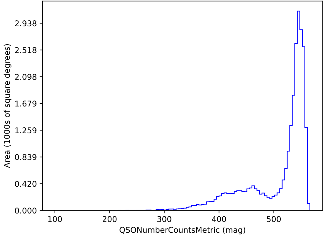
roll_uniform_early_half_mjdp180_v3.4_10yrs i band and non-DD: QSONumberCountsMetric
