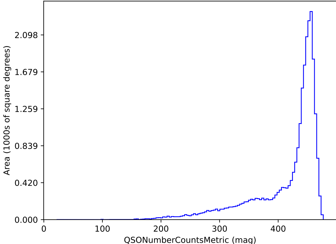
roll_uniform_early_half_mjdp180_v3.4_10yrs g band and non-DD: QSONumberCountsMetric
