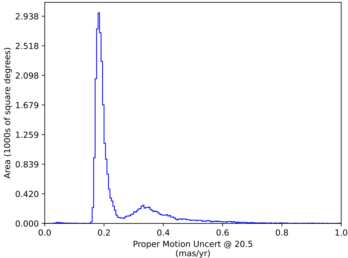
roll_uniform_early_half_mjdp180_v3.4_10yrs : Proper Motion Uncert @ 20.5
