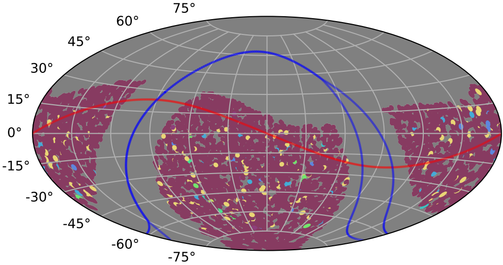
roll_uniform_early_half_mjdp180_v3.4_10yrs : PrestoKNe_score_p
