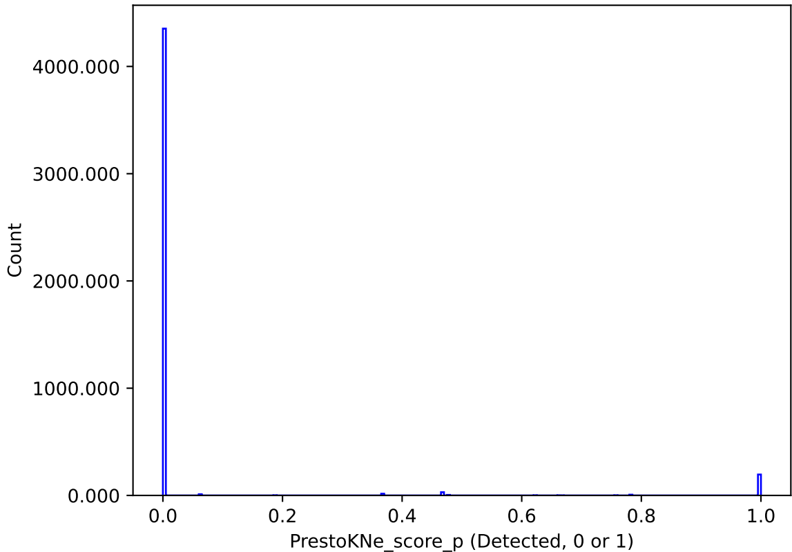
roll_uniform_early_half_mjdp180_v3.4_10yrs : PrestoKNe_score_p
