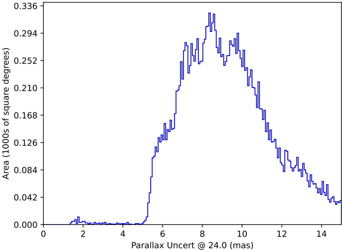
roll_uniform_early_half_mjdp180_v3.4_10yrs : Parallax Uncert @ 24.0
