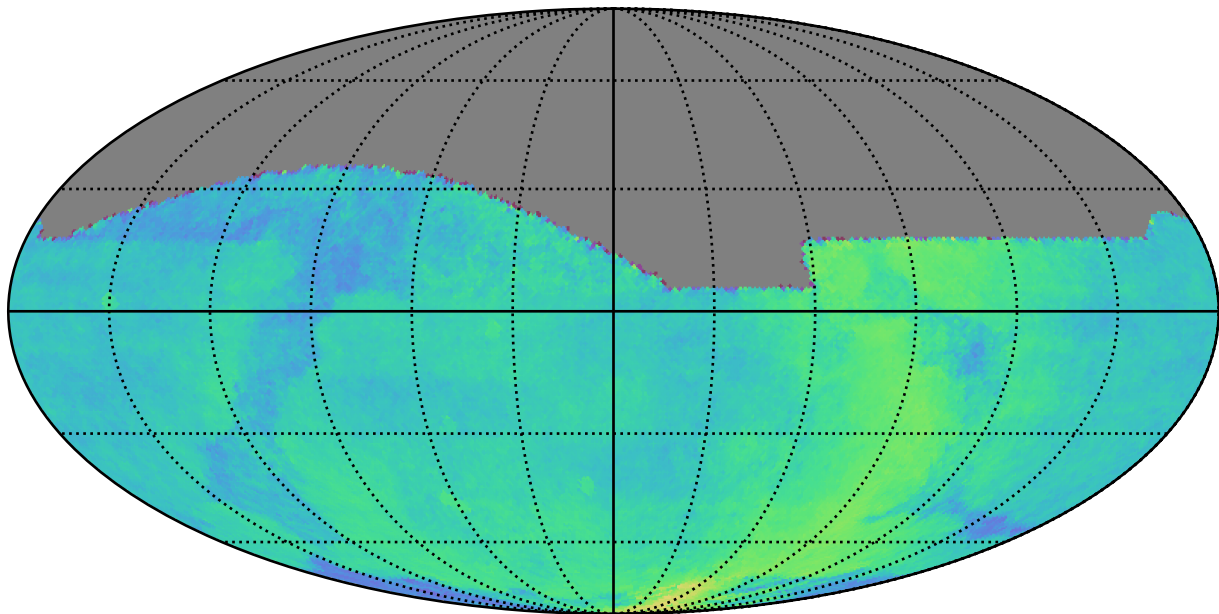
roll_uniform_early_half_mjdp180_v3.4_10yrs : Parallax Coverage @ 22.4
