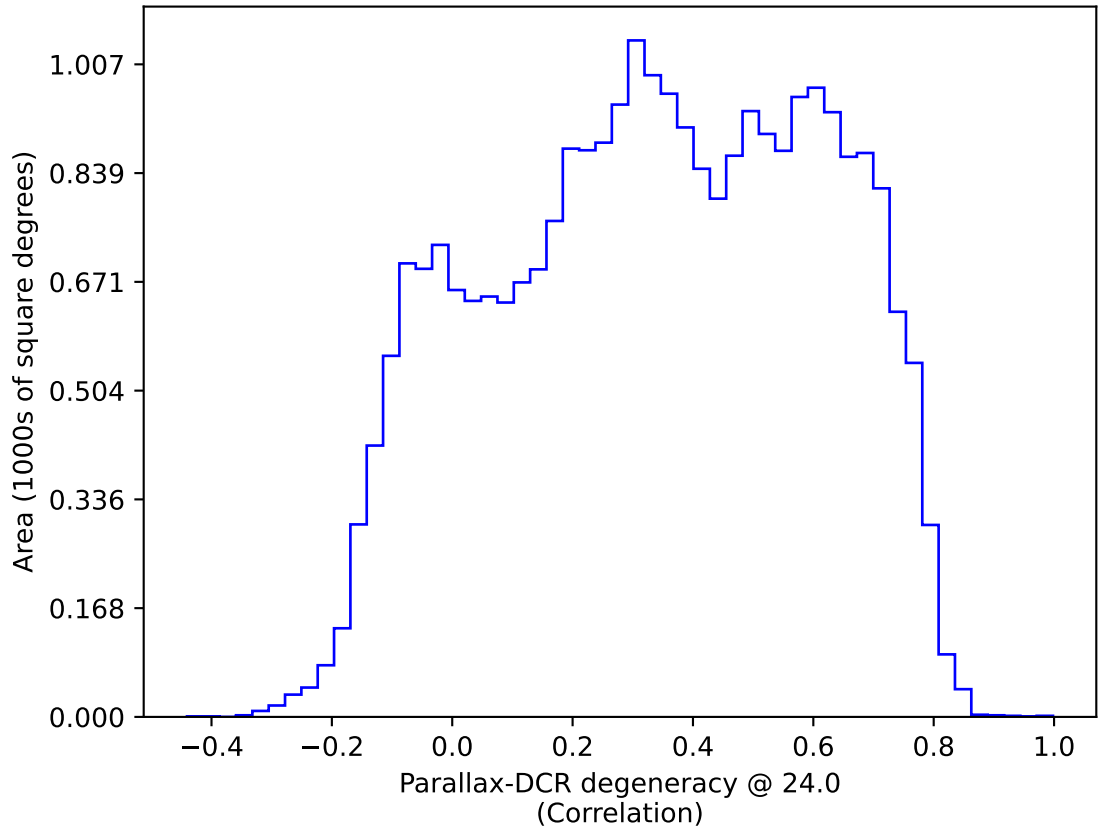
roll_uniform_early_half_mjdp180_v3.4_10yrs : Parallax-DCR degeneracy @ 24.0
