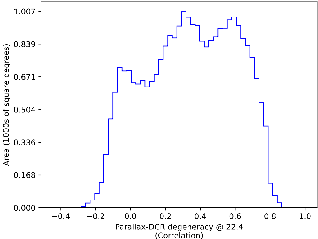
roll_uniform_early_half_mjdp180_v3.4_10yrs : Parallax-DCR degeneracy @ 22.4
