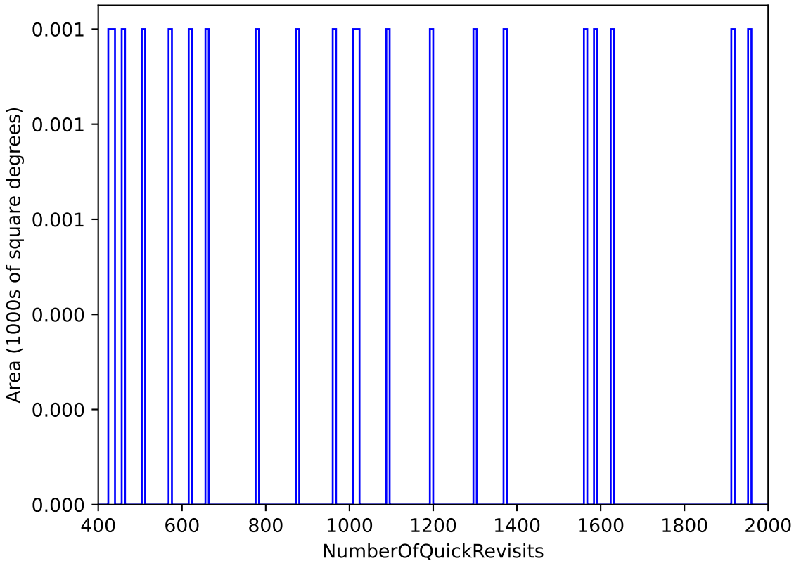
roll_uniform_early_half_mjdp180_v3.4_10yrs : NumberOfQuickRevisits
