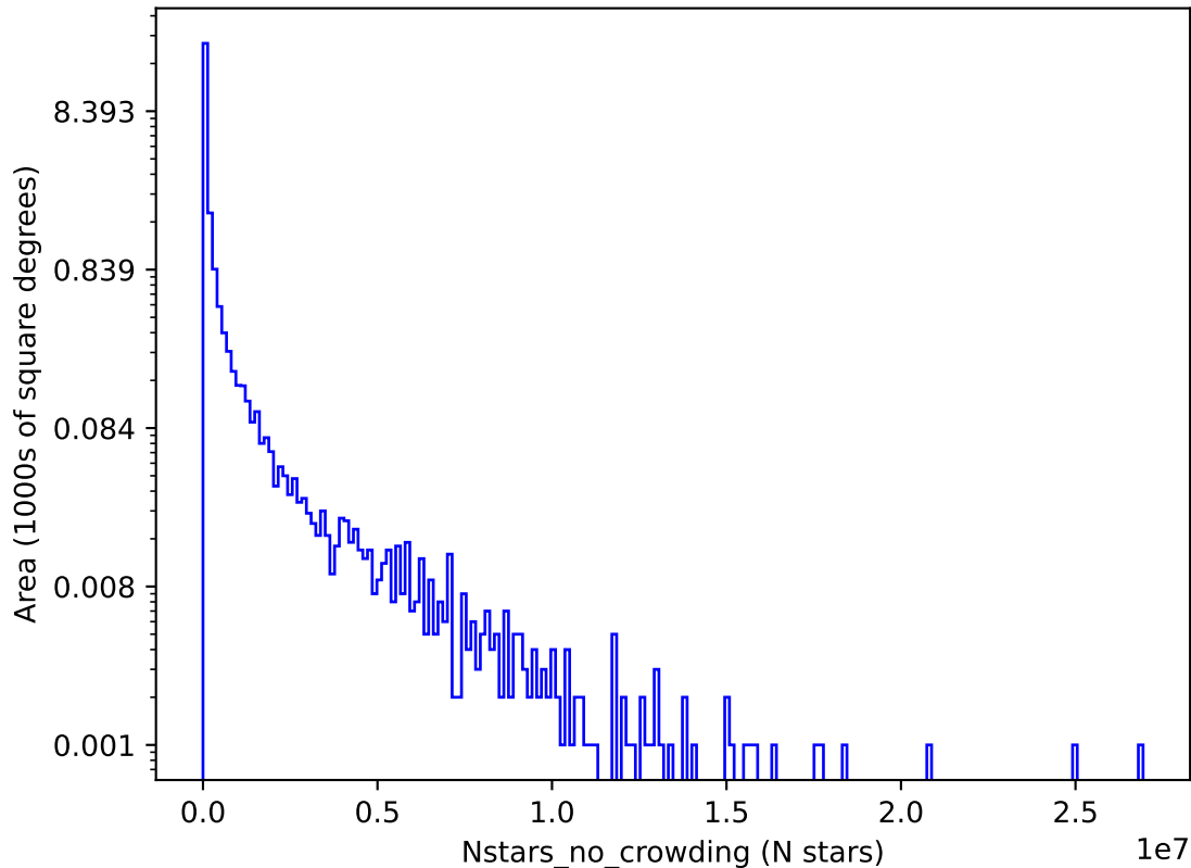
roll_uniform_early_half_mjdp180_v3.4_10yrs i: Nstars_no_crowding
