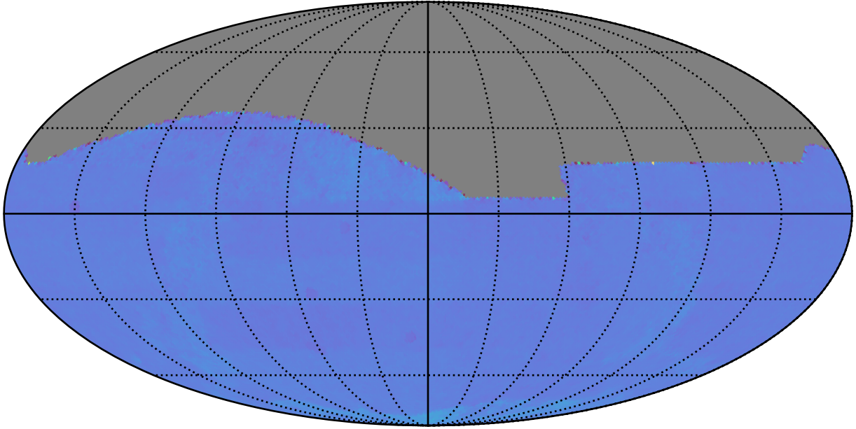
roll_uniform_early_half_mjdp180_v3.4_10yrs : Normalized Proper Motion Uncert @ 20.5
