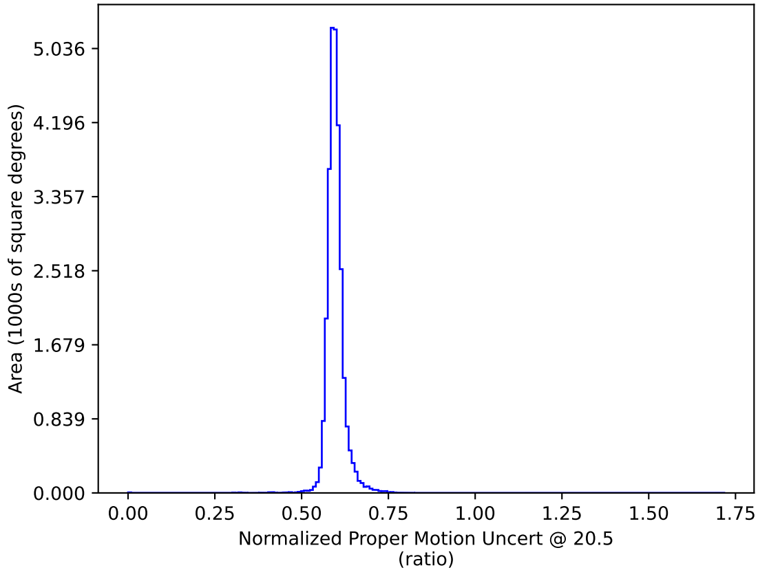
roll_uniform_early_half_mjdp180_v3.4_10yrs : Normalized Proper Motion Uncert @ 20.5
