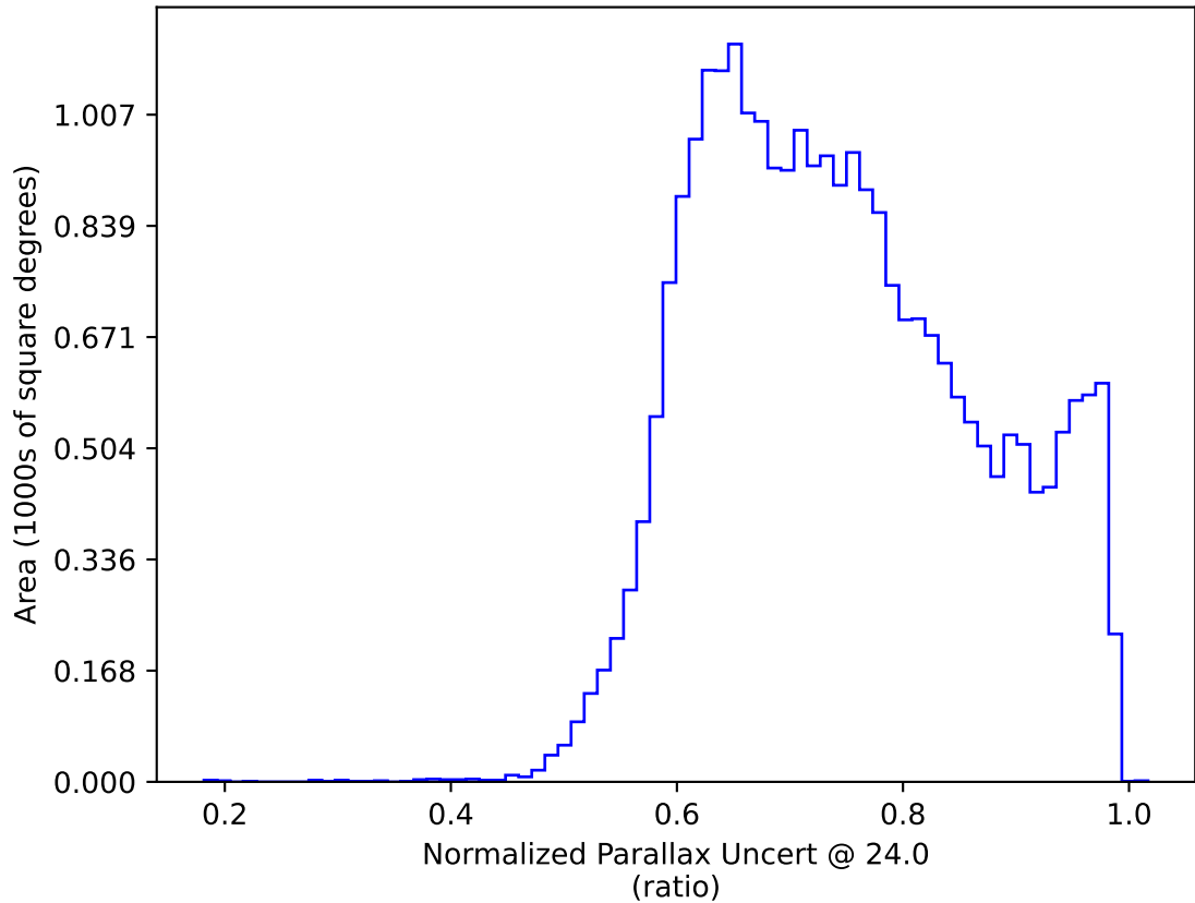
roll_uniform_early_half_mjdp180_v3.4_10yrs : Normalized Parallax Uncert @ 24.0
