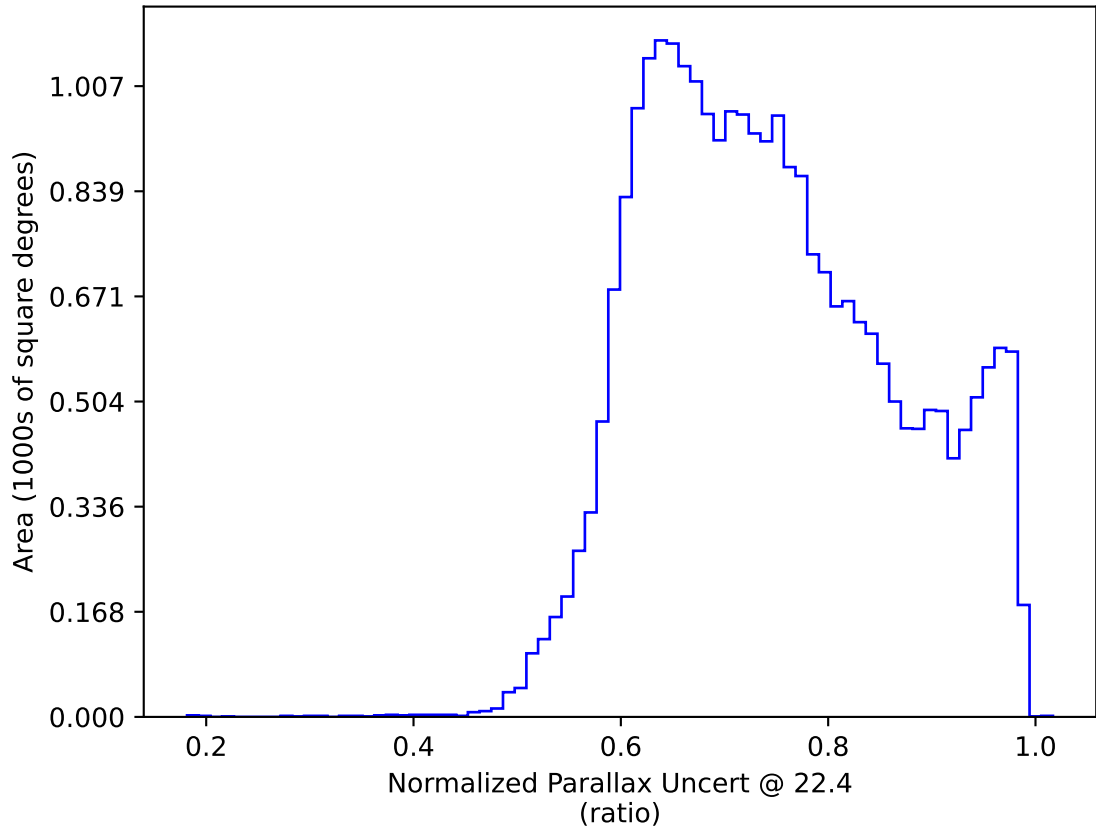
roll_uniform_early_half_mjdp180_v3.4_10yrs : Normalized Parallax Uncert @ 22.4
