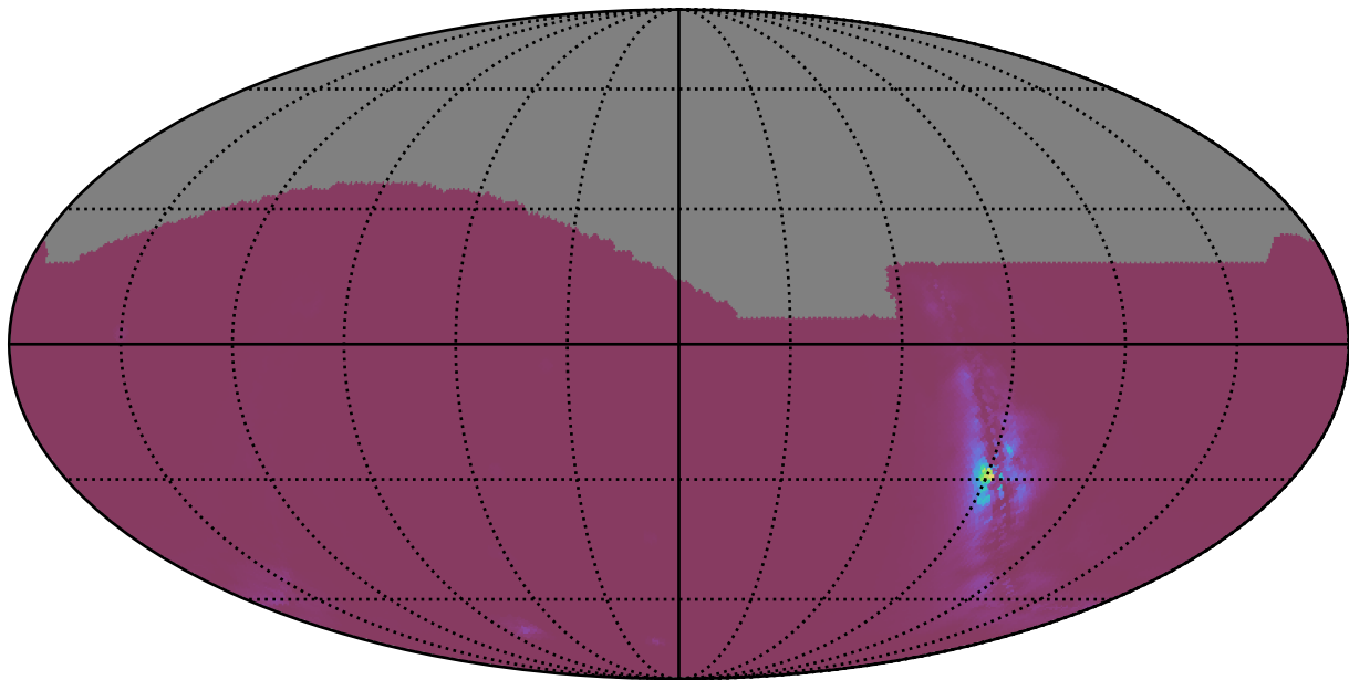
roll_uniform_early_half_mjdp180_v3.4_10yrs : NlcPoints
