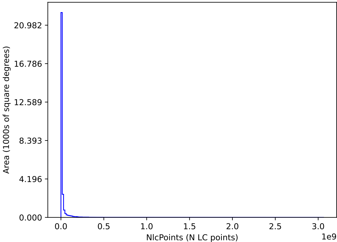
roll_uniform_early_half_mjdp180_v3.4_10yrs : NlcPoints
