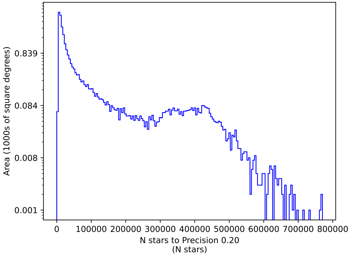
roll_uniform_early_half_mjdp180_v3.4_10yrs r: N stars to Precision 0.20
