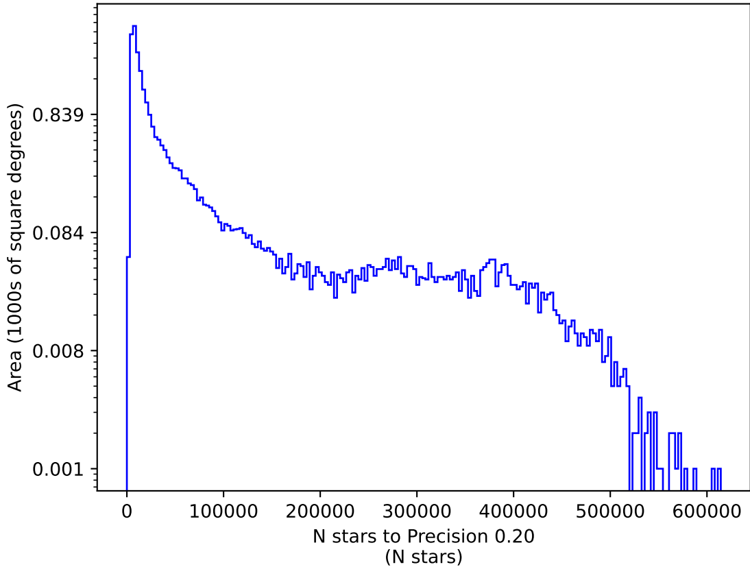
roll_uniform_early_half_mjdp180_v3.4_10yrs g: N stars to Precision 0.20
