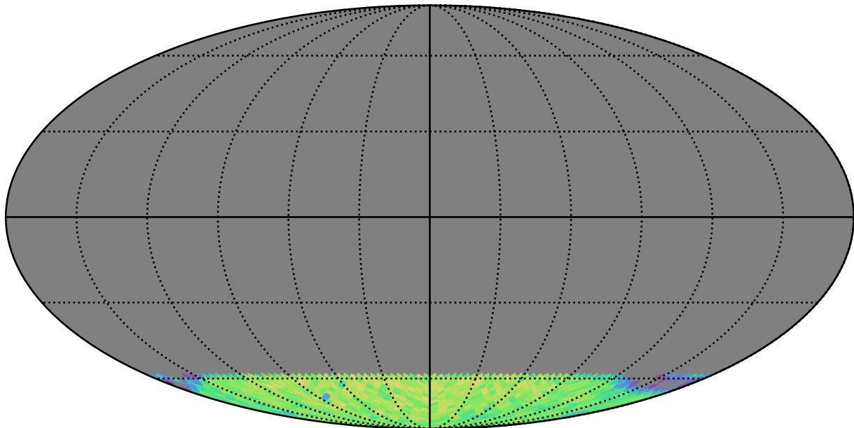
roll_uniform_early_half_mjdp180_v3.4_10yrs gi SCP: LVDwarfs
