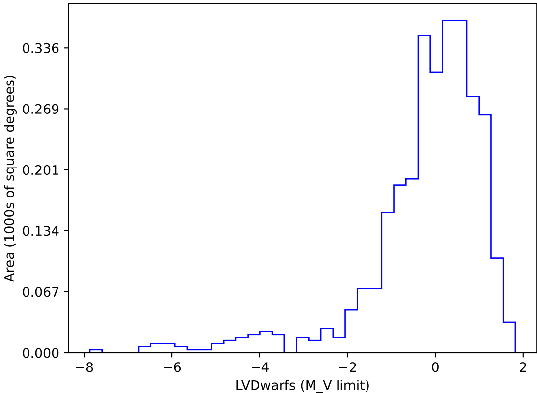
roll_uniform_early_half_mjdp180_v3.4_10yrs gi SCP: LVDwarfs
