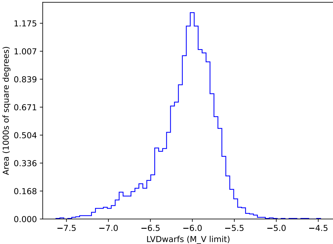
roll_uniform_early_half_mjdp180_v3.4_10yrs gi: LVDwarfs
