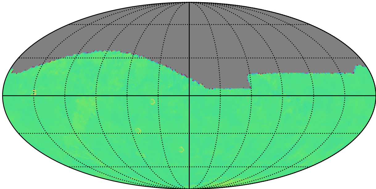
roll_uniform_early_half_mjdp180_v3.4_10yrs r: Kuiper rotTelPos
