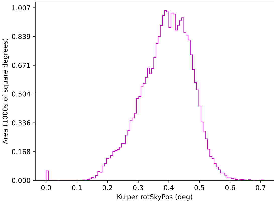
roll_uniform_early_half_mjdp180_v3.4_10yrs z: Kuiper rotSkyPos
