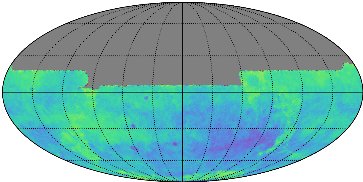
roll_uniform_early_half_mjdp180_v3.4_10yrs y: Kuiper rotSkyPos
