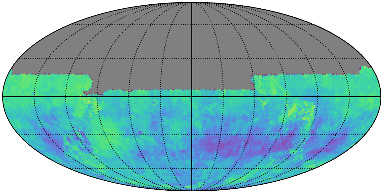
roll_uniform_early_half_mjdp180_v3.4_10yrs u: Kuiper rotSkyPos
