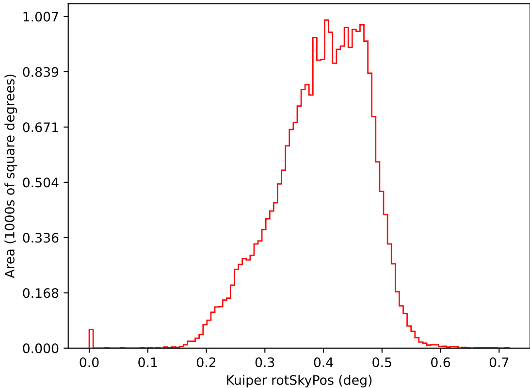
roll_uniform_early_half_mjdp180_v3.4_10yrs i: Kuiper rotSkyPos
