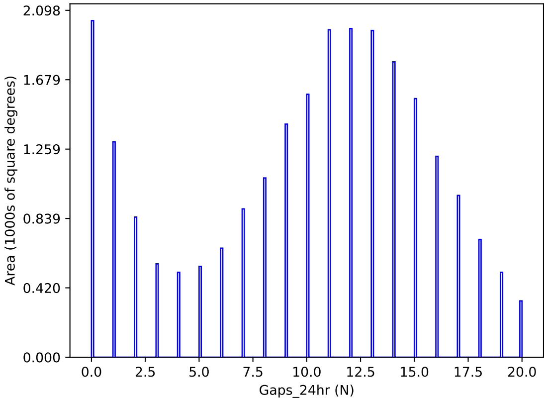
roll_uniform_early_half_mjdp180_v3.4_10yrs y band: Gaps_24hr
