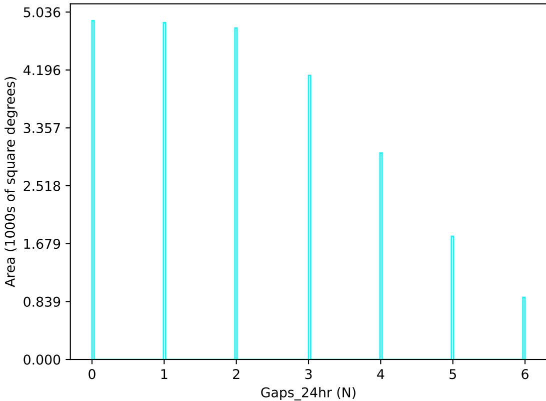
roll_uniform_early_half_mjdp180_v3.4_10yrs u band: Gaps_24hr
