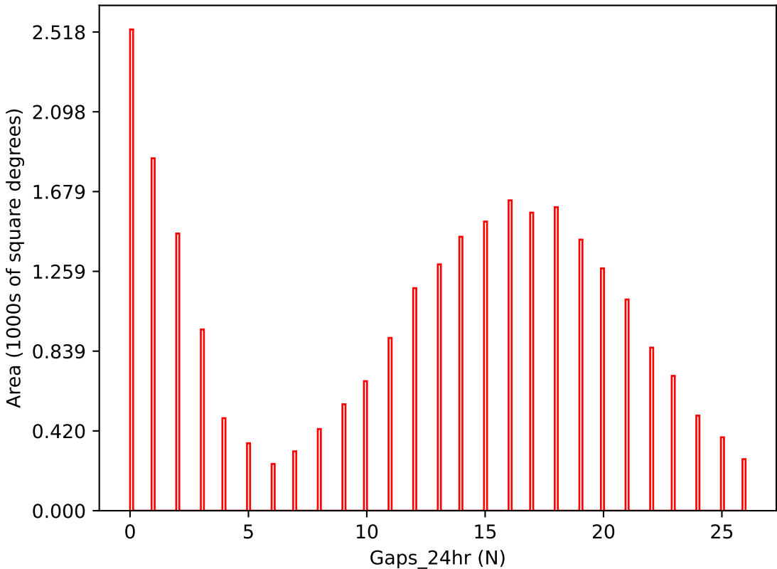
roll_uniform_early_half_mjdp180_v3.4_10yrs i band: Gaps_24hr
